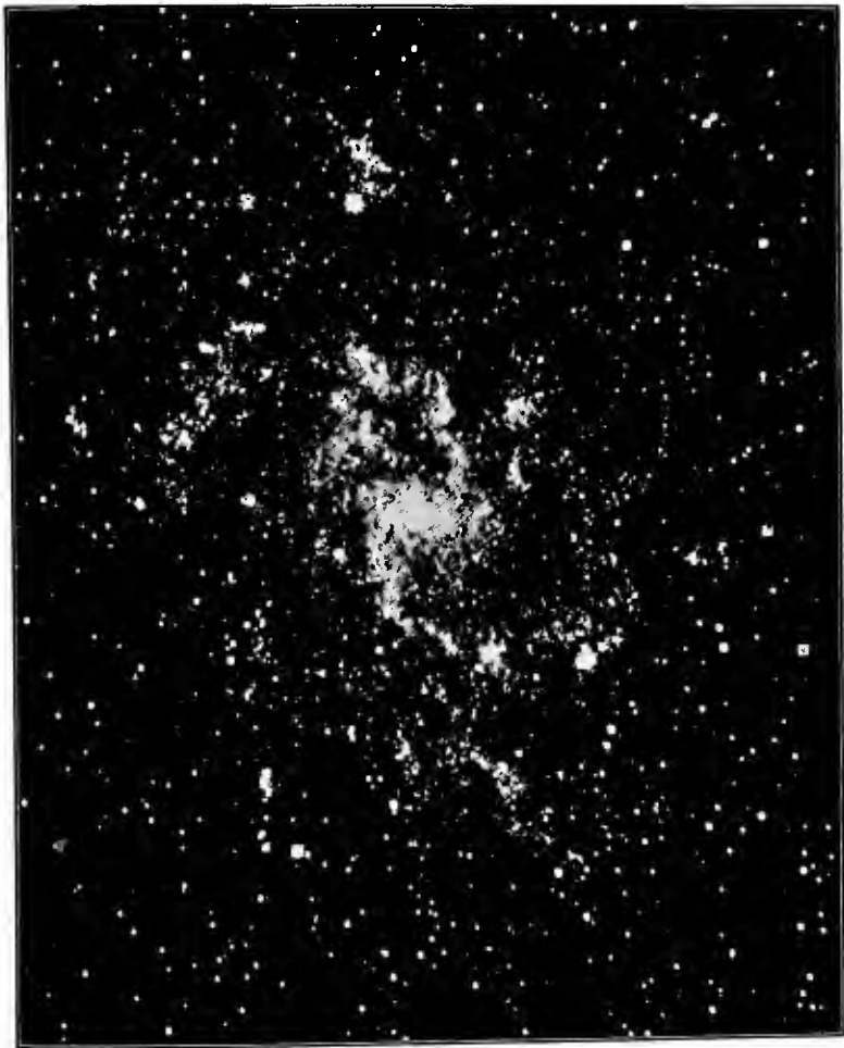
WONDERFUL SPIRAL IN TRIANGULUM
